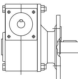
Output flange
